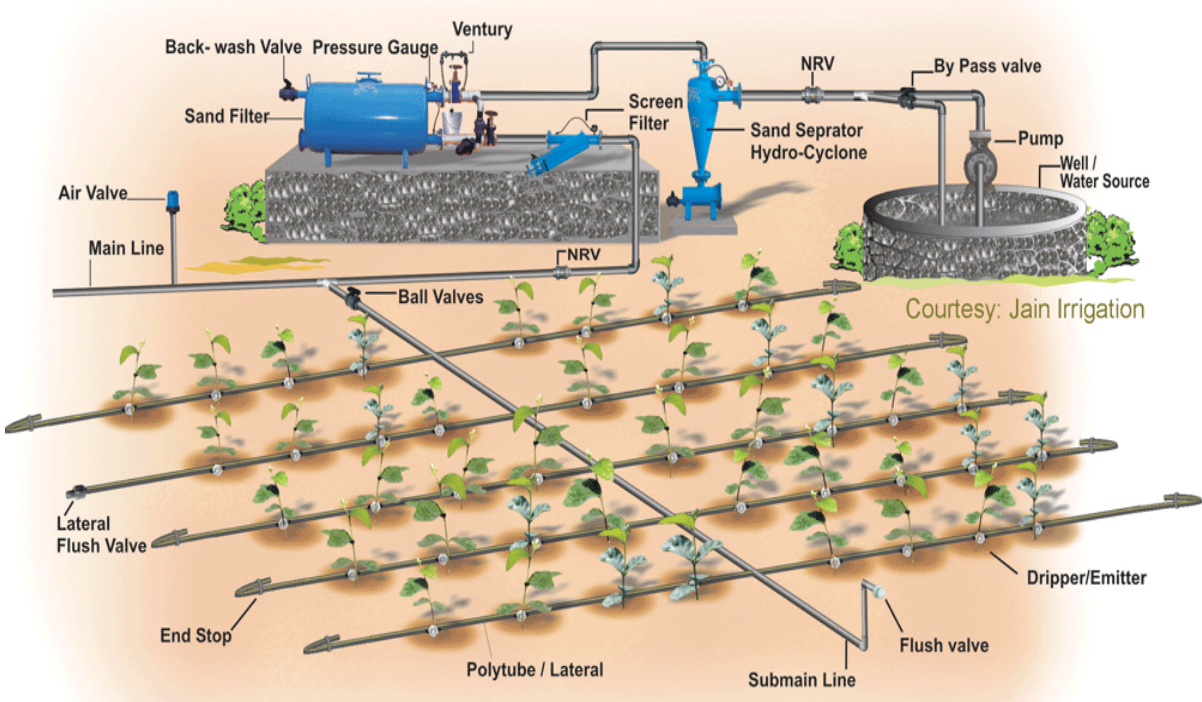
Drip irrigation system
