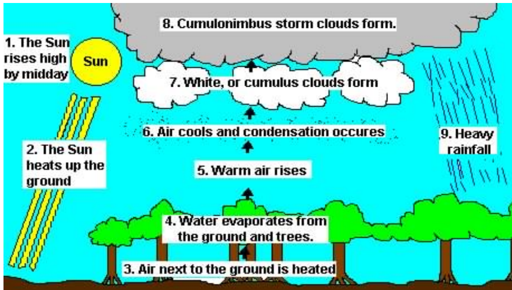
CONVECTIONAL RAIN FALL
