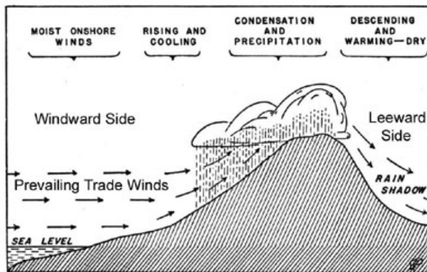
OROGRAPHIC RAINFALL
