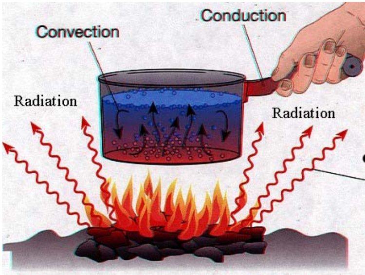
CONDUCTION, CONVECTION AND RADIATION
