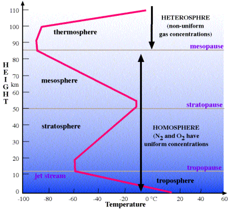
TEMPERATURE CHANGES WITH ALTITUDE
